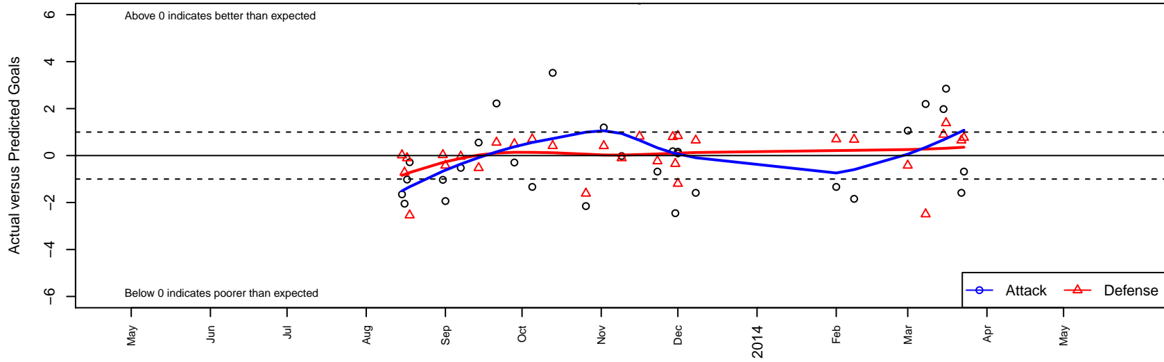
LWPFC White Stingrays G02 Dots are actual minus expected GF (blue circles) and GA (red triangles). Blue line is smoothed change in attack strength. Red is smoothed change in defense strength.
